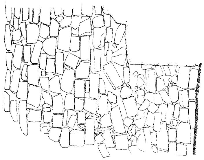
Façade K-K
